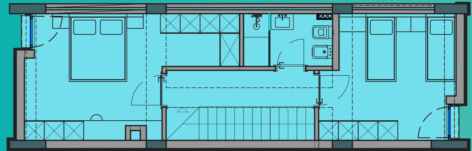
FIRST FLOOR
