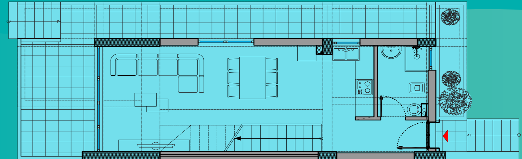
FIRST FLOOR
