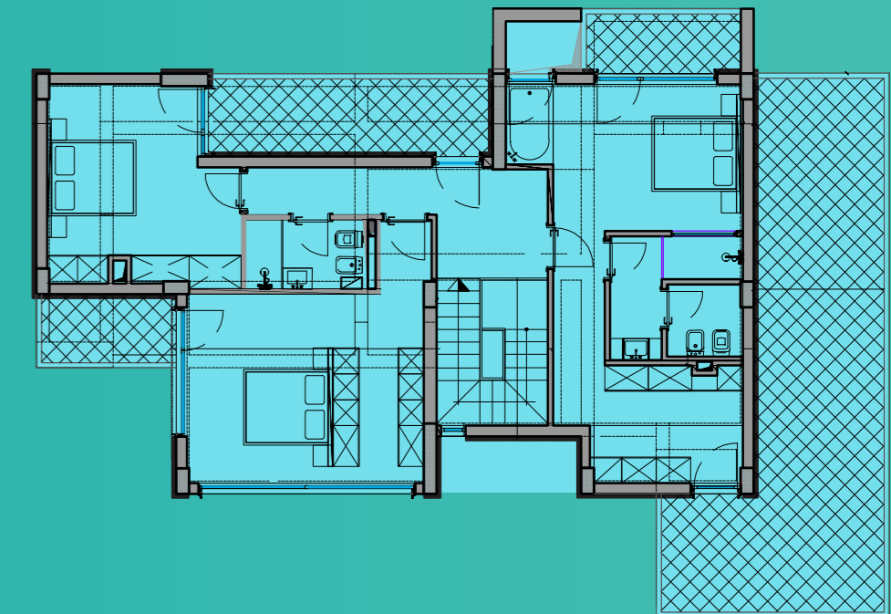
FIRST FLOOR
